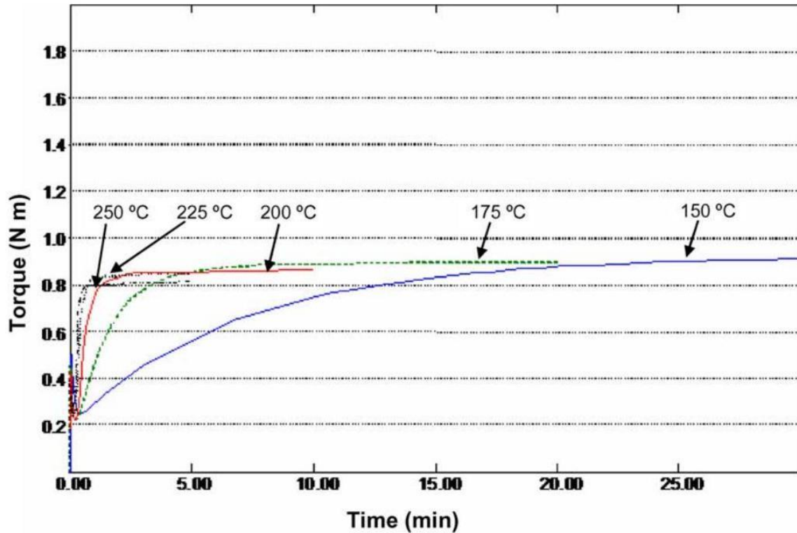
Fig. 7. Rheometer curves for thermoset crosslinking of EPDM with SnCl 2 -activated resol at different temperatures ( 150,175,200,225 and 250 °C ).
