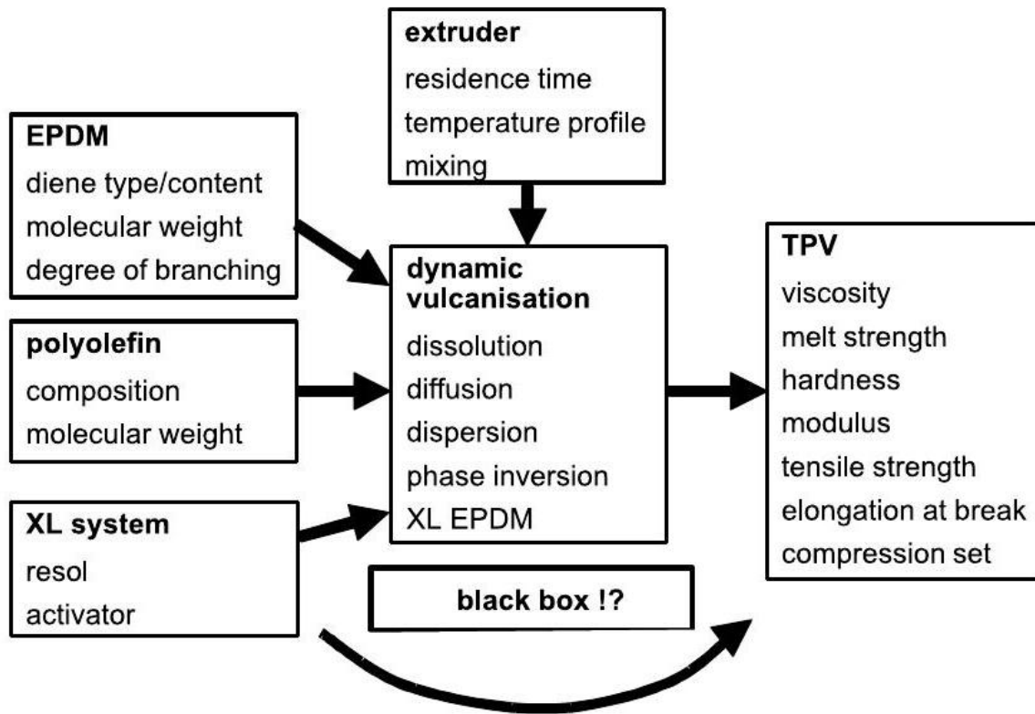
Fig. 1. Schematic representation of dynamic vulcanisation of rubber/thermoplastic blends, yielding thermoplastic vulcanisates. the highest volume fraction becomes the matrix and the phase with the highest viscosity and/or the lowest volume fraction the dispersion [12]. At similar viscosities and/or equal volume fractions a co-continuous morphology is obtained. Although refined theories have been developed in the last decade to predict blend morphologies [15-17], it is felt that the basic Avgeropoulos model is sufficient to explain phase inversion during TPV production. Romanini was the first to use this model to explain the morphology of TPVs [8]. Crosslinking of the rubber results in an increase of the viscosity of the rubber phase and, thus, in phase inversion. Abdou-Sabet and Patel gave experimental evidence by 'mapping' the Avgeropoulos plot for EPDM/ PP blends with a large variation in composition and EPDMs with different viscosities [9]. Radusch and Pham developed a mathematical model predicting the morphology of TPVs by combining mixing, mass and heat transport with crosslinking kinetics [10]. Recently, several studies have shown that not simply the change in melt viscosity, but the change in elasticity of the rubber phase is the driving force for phase inversion [13,14].
