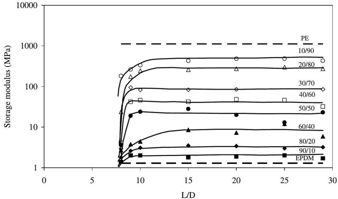
Fig. 5. Storage modulus measured at room temperature of EPDM/PE ( 90/10 to 10/90; w/w) TPVs with crosslinking as a function of screw length. content was used to study the degree of crosslinking along the screw axis, and TEM was used to determine the actual morphology.
