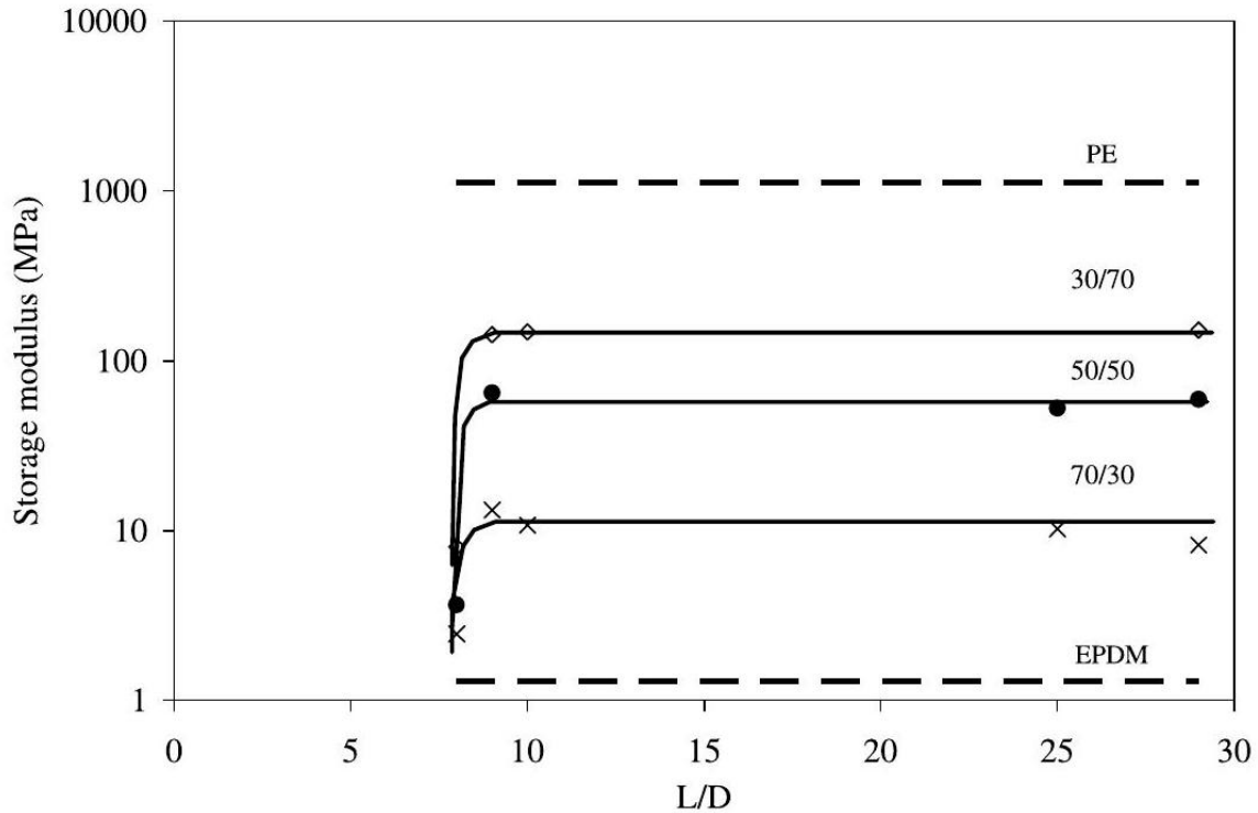
Fig. 4. Storage modulus measured at room temperature of EPDM/PE (70/30, 50/50 and 30/70; w/w) blends without crosslinking as a function of screw length. L/D = 8 and for the PE-rich TPVs (20/80 and 10/90; w/w) at L/D = 9 (indicated by the dashed, vertical line in Fig. 3). However, substantial amounts of the PE pellets are molten at L/D = 8 , because the quenched melt samples feel rather rigid, indicating the presence of PE next to that of EPDM. Considering that the melting point of HDPE is about 120^{\circ}\text{C} , the presence of non-molten PE pellets at L/D = 8 and 9, where melt temperatures of 200^{\circ}\text{C} and higher are measured, shows that the samples are not in equilibrium with respect to heat transfer. The higher the PE content of the TPVs (20/80 and 10/90; w/w), which also corresponds to the lower the melt temperature ( \sim 200^{\circ}\text{C} ), the longer it takes before the samples are homogeneous with respect to heat transfer (up to L/D = 9 ).
