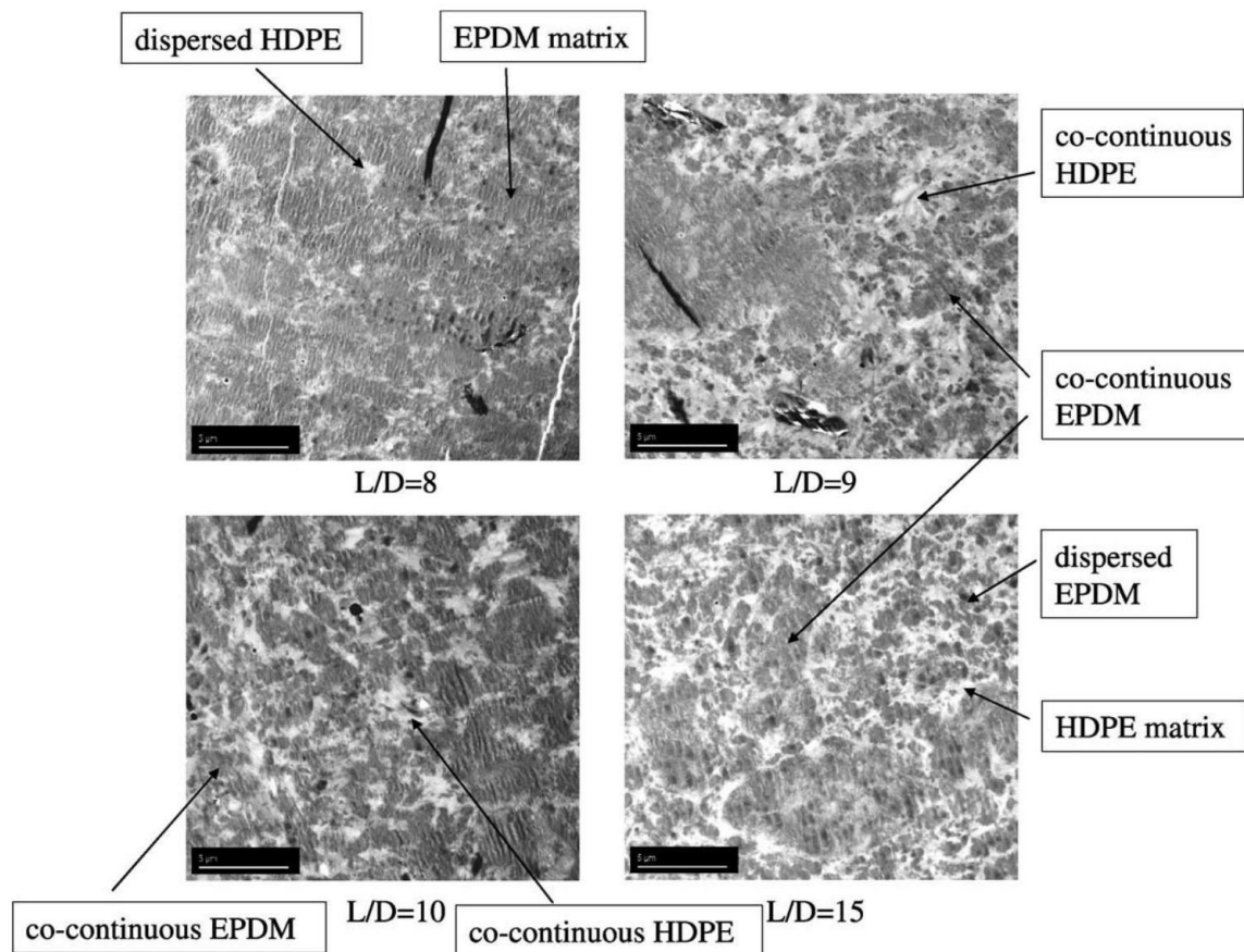
Fig. 11. TEM micrographs of EPDM/PE (50/50; w/w) TPVs at L/D = 8, 9, 10 and 15 . temperature. For the TPVs high degrees of crosslinking are already observed in the first kneading section. As a result, the EPDM viscosity increases strongly and, consequently, the melt temperature increases to values (far) above the barrel set temperature. The higher the EPDM content of the TPVs, the higher the viscous dissipation during extrusion, the higher the rise of the temperature and, thus, the higher the crosslinking rate. So, there is a reciprocal interaction between the melt temperature and crosslinking. Only for the PE-
