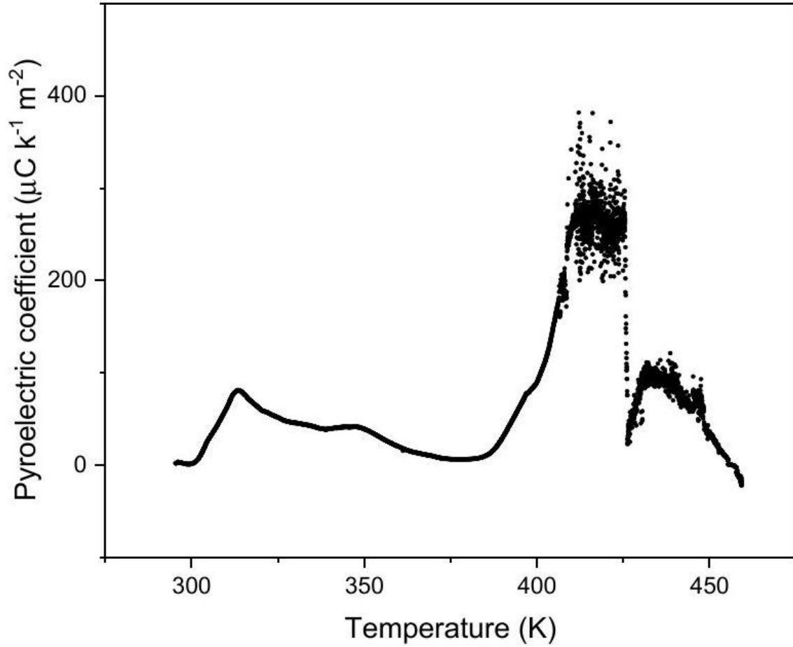
Figure 2. Pyroelectric coefficient as a function of the temperature of MDABCO- \text{NH}_4\text{Cl}_3 , measured during heating.
