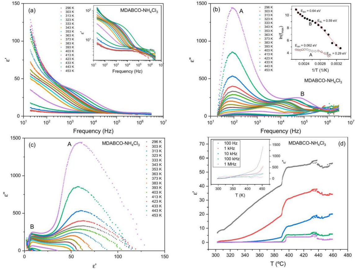
Figure 1. Frequency dependence of the (a) real part and (b) imaginary part of the dielectric permittivity polycrystalline MDABCO- \text{NH}_4\text{Cl}_3 . (b) Inset plots of the logarithm of the frequency corresponding to the maximum of the relaxations marked with A (open dots) and B (closed dots) in \epsilon'' versus the inverse of the temperature. The straight red lines are fits to the curves, which were used to obtain the corresponding activation energies. (c) The Cole-Cole plot and (d) temperature dependence of the real and imaginary (inset) components of the electric permittivity of the sample.
