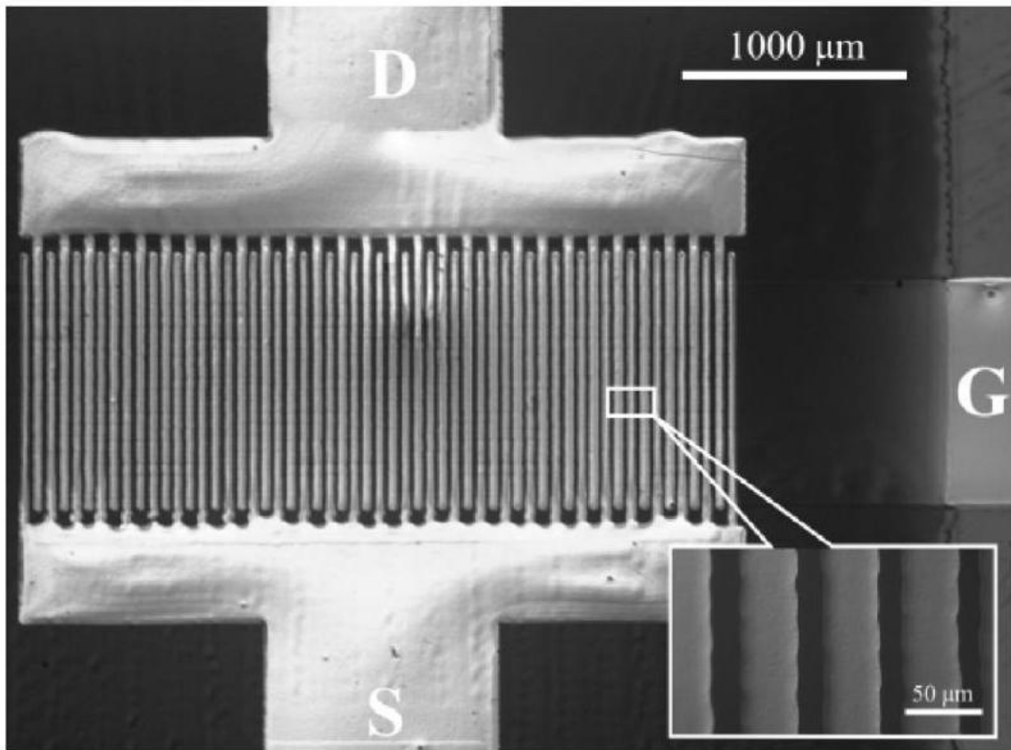
Fig. 2. Optical microscope image of the all-inkjet-printed OTFT structure with channel ratio W/L = 61,600/15\mu\text{m} . voltage and subthreshold swing were 0.198\text{ cm}^2\text{ V}^{-1}\text{ s}^{-1} , 8 \times 10^3 , 3.15\text{ V} , and 3.2\text{ V/dec} . Fig. 3 c and d shows the transfer and output characteristics of the OTFTs with the W/L ratio of 61,600\mu\text{m}/15\mu\text{m} . The average values of field effect mobility, on/off ratio, threshold voltage and subthreshold swing are 0.076\text{ cm}^2\text{ V}^{-1}\text{ s}^{-1} , 1.4 \times 10^5 , 4.05\text{ V} , and 2.2\text{ V/dec} , respectively.
