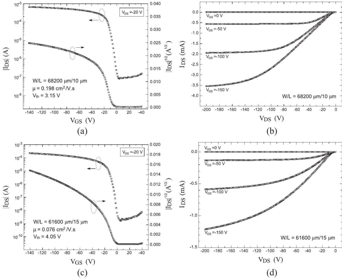
Fig. 3. Electrical characteristics of all-inkjet-printed OTFTs without any treatment. (a) Transfer and (b) output characteristics of the TFTs with W/L ratio of 68,200\mu\text{m}/10\mu\text{m} . (c) Transfer and (d) output characteristics of the OTFTs with a W/L ratio of 61,600\mu\text{m}/15\mu\text{m} .
