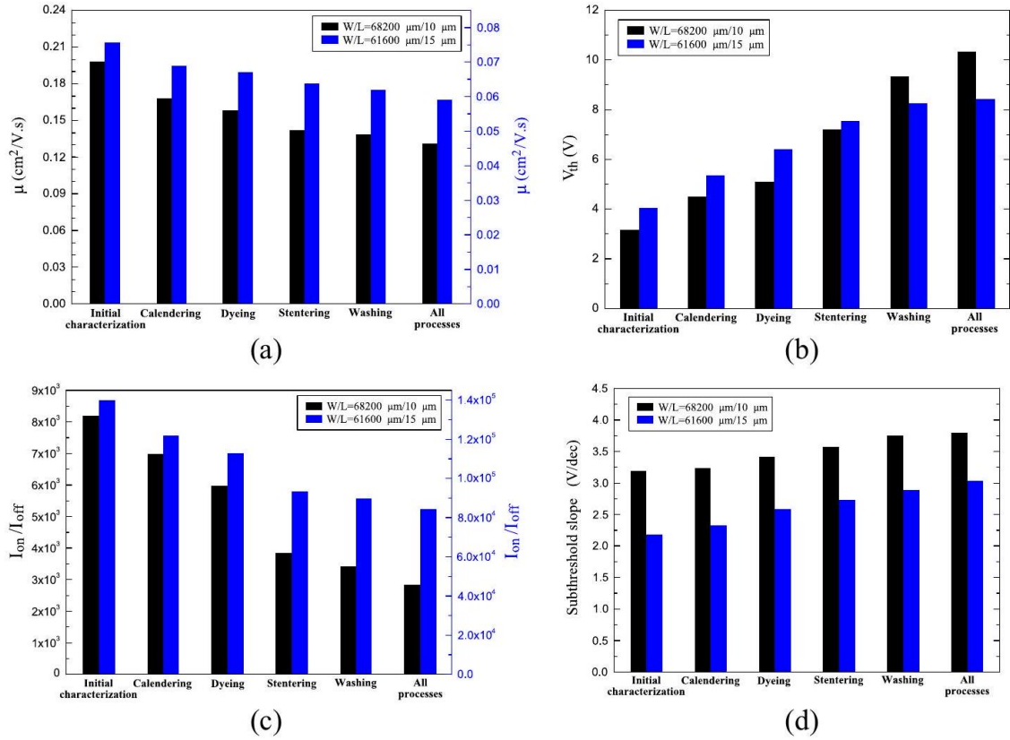
Fig. 6. Comparison of the (a) field effect mobility, (b) threshold voltage, (c) on/off ratio, and (d) subthreshold slope of the OTFTs with a W/L ratio of 68,200 \mu\text{m}/10 \mu\text{m} and W/L ratio of 61,600 \mu\text{m}/15 \mu\text{m} as a function of treatment process applied in textile manufacturing.
