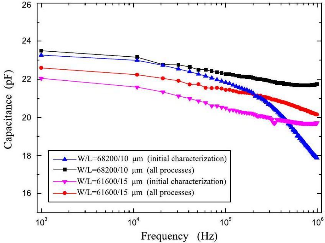
Fig. 4. Overlap capacitance as a function of frequency for the all-inkjet-printed OTFT with the channel ratio of W/L = 68,200\mu\text{m}/10\mu\text{m} and W/L = 61,600/15\mu\text{m} . process (each graph is an average of data from three OTFTs). Both individual treatment processes as well as the sequence of all treatment processes are considered and compared with the OTFTs performance without any treatment (initial characterization). As can be observed the OTFTs maintain their basic electrical functionality in all cases. The treatment processes did not destroy the OTFTs, e.g. by short circuits due to a defective dielectric and similar reasons. However, there is a noticeable degradation of the electrical characteristics which depends on the textile process and the W/L ratio. The degradation seems to be more prominent for a W/L ratio of 68,200\mu\text{m}/10\mu\text{m} as compared to 61,600\mu\text{m}/15\mu\text{m} . Furthermore, the highest degradation is observed as expected when subjecting the OTFTs to all processes in a sequence.
