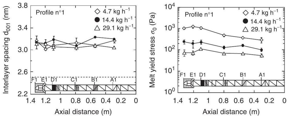
Figure 10.5 Effect of feed rate on the variation along the extruder of interlayer spacing (a) and melt yield stress (b). Reproduced with permission from [14] © 2007, Society of Plastics Engineers.
