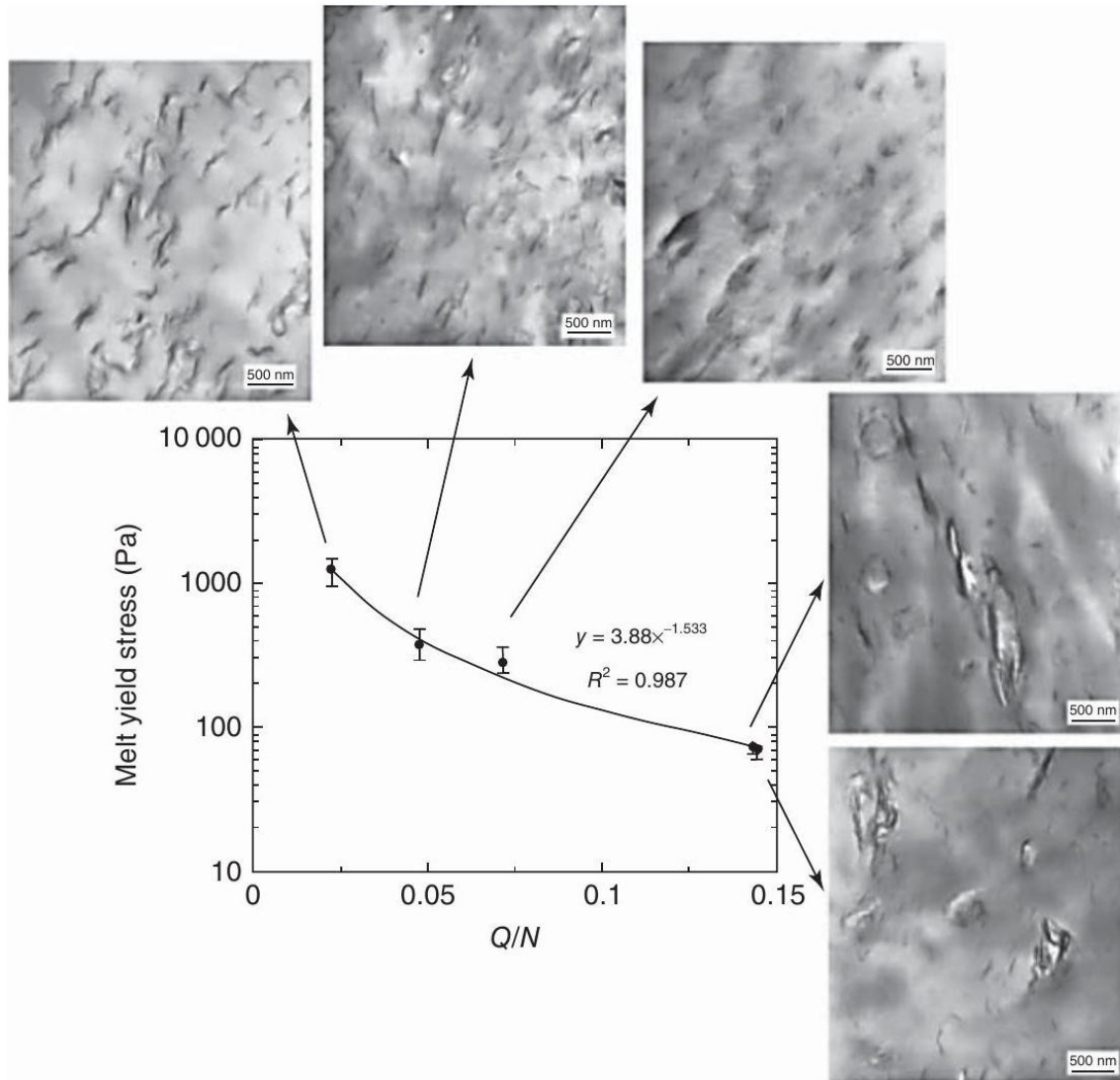
Figure 10.3 Evolution of melt yield stress as a function of filling ratio (output/screw speed, Q/N) for PP-clay nanocomposites prepared under different operating conditions. Reproduced with permission from [12] © 2006, Society of Plastics Engineers.
