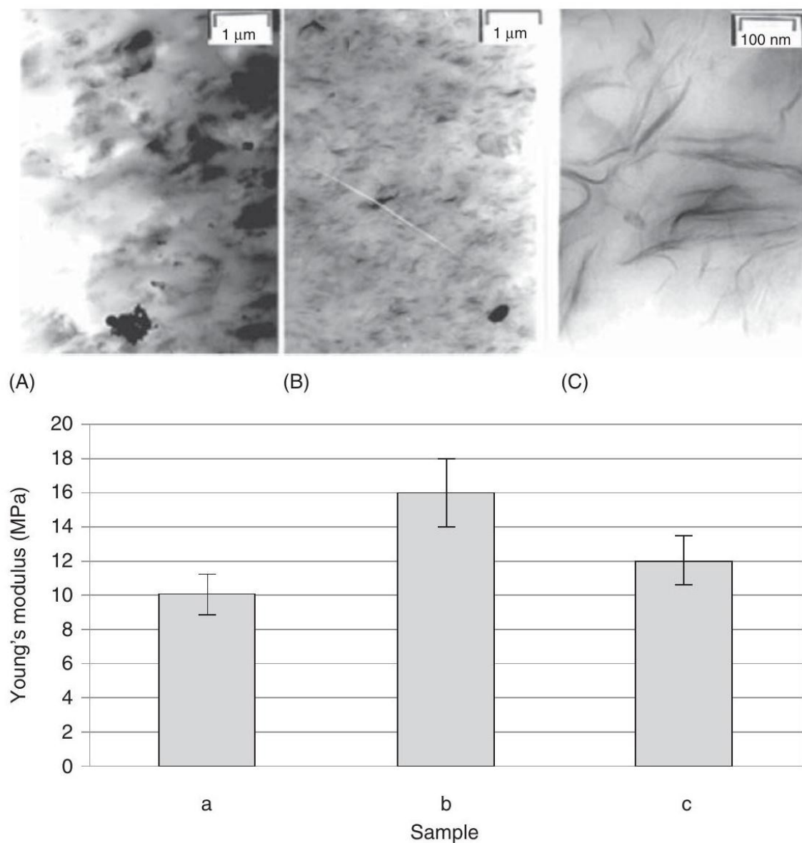
Figure 10.4 Polymer-clay nanocomposite showing different dispersion levels and respective Young's modulus. Reproduced with permission from [11] © 2006, American Chemical Society.
