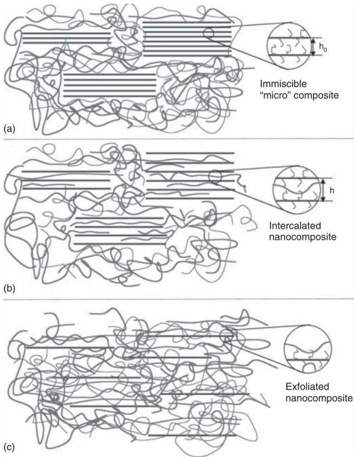
Figure 10.1 (a-c) Possible polymer-clay nanocomposite morphologies. Reproduced with permission from [9] © 2001, AIP Publishing LLC.
