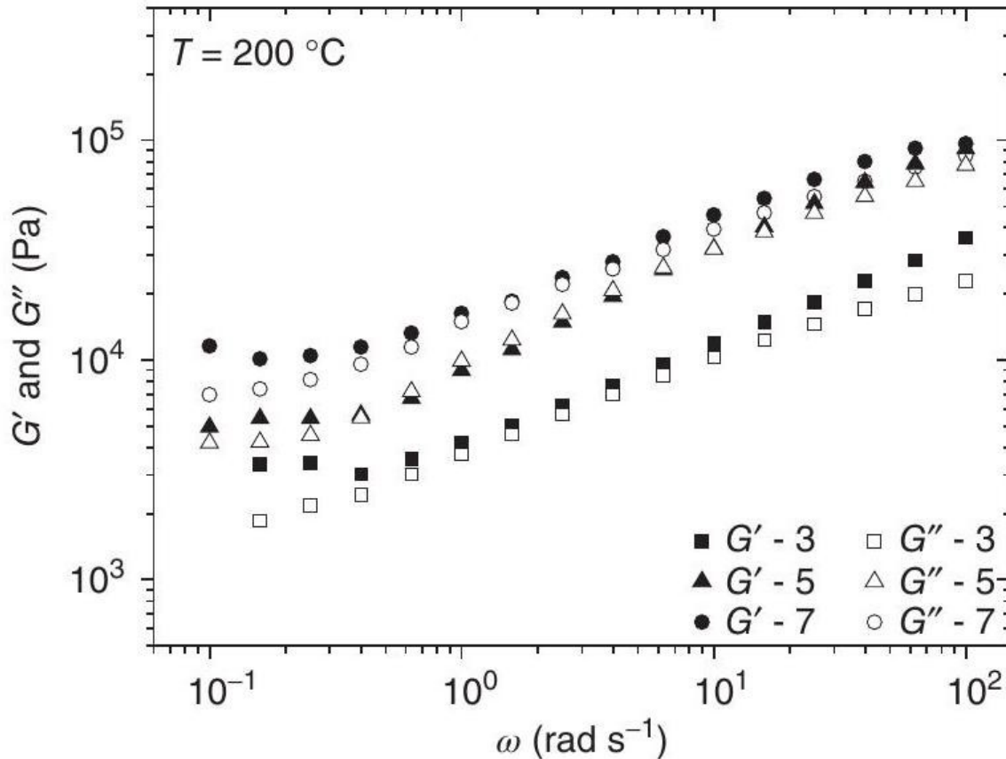
Figure 10.6 Linear viscoelastic behavior of PP/PP-g-MA/D67G nanocomposite at 200 °C, measured online at three axial locations ( 3,5 , and 7, in the downstream direction) along a corotating twin screw extruder [76].
