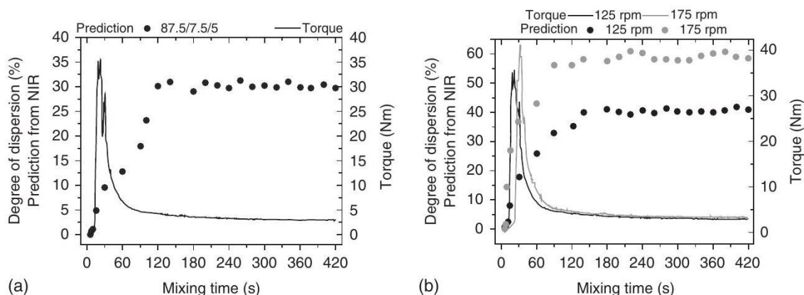
Figure 10.8 Evolution of torque and (predicted) average dispersion with mixing time during the preparation of a PP/PP-g-MA/Closite 20A nanocomposite in a Haake mixer: (a) 87.5/7.5/5 w/w % at 50 rpm and (b) 90/5/5 % at 125 and 175 rpm
